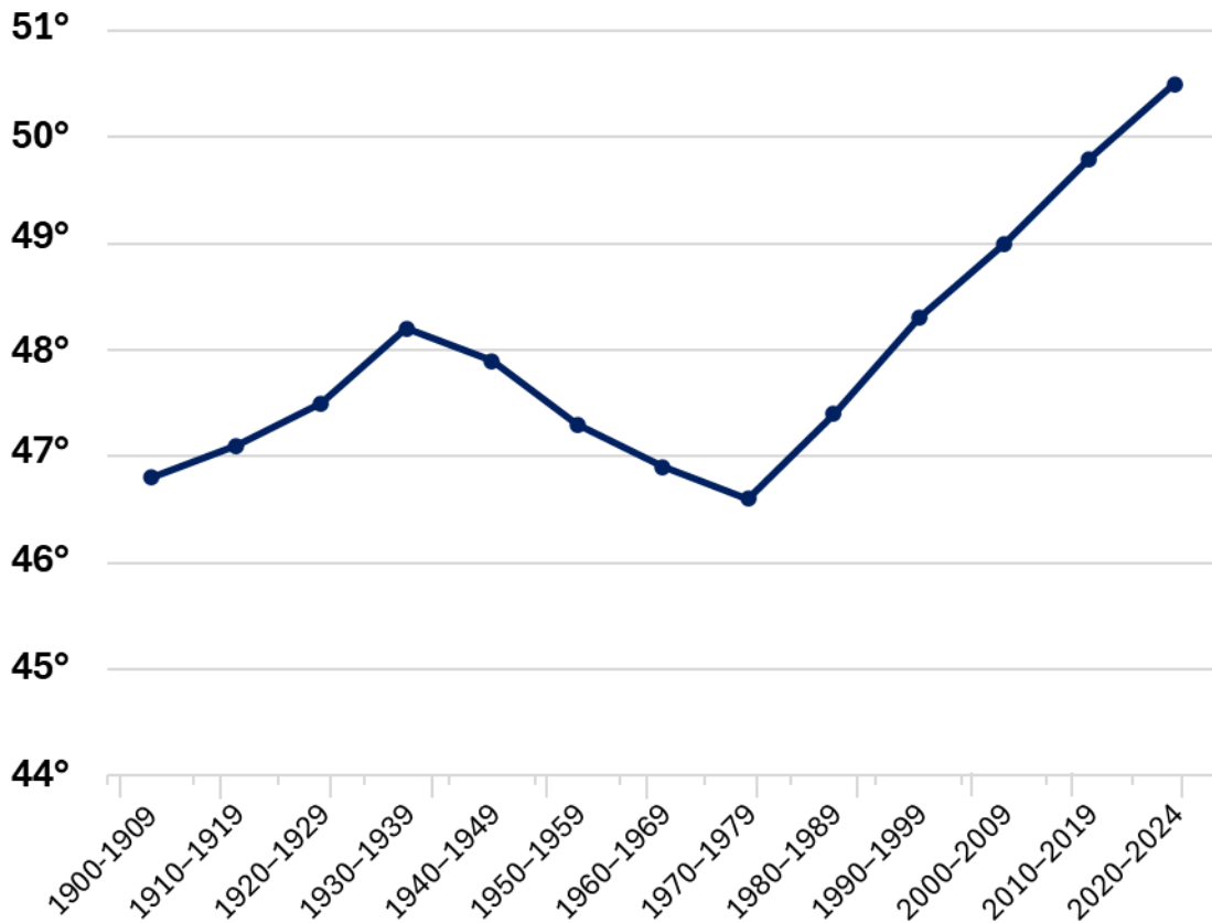
Figure 2. Erie County NY, Average Temperature by Decade
