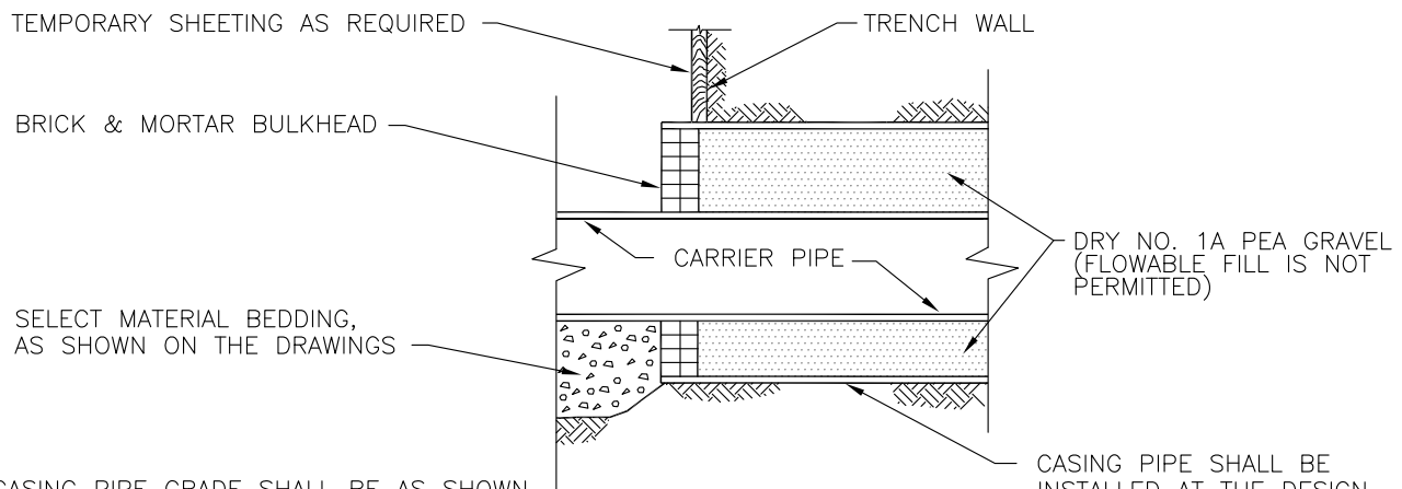
SECTION B-B CASING PIPE DETAILS
