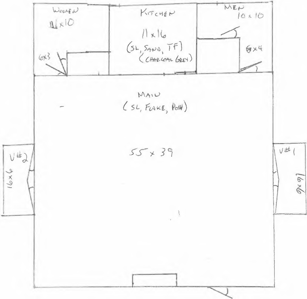
Emery Park Strohrer's Lodge sketch:
